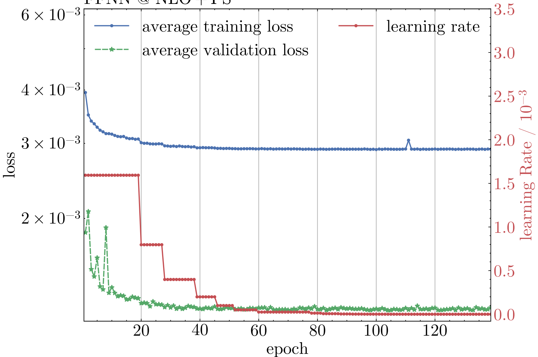
FFNN @ NLO + PS
