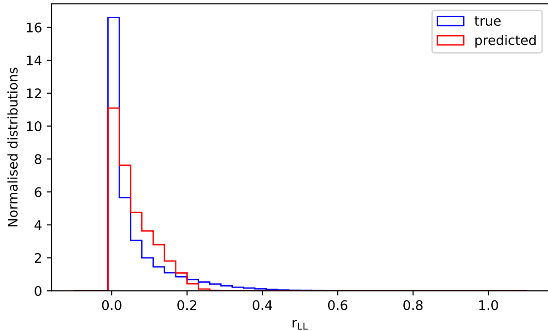
Label distribution
