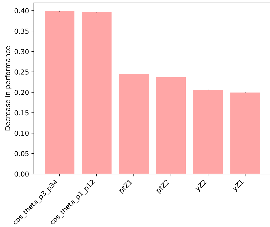
Permutation importance for RFR ct (NLO QCD, LHE, fiducial)
