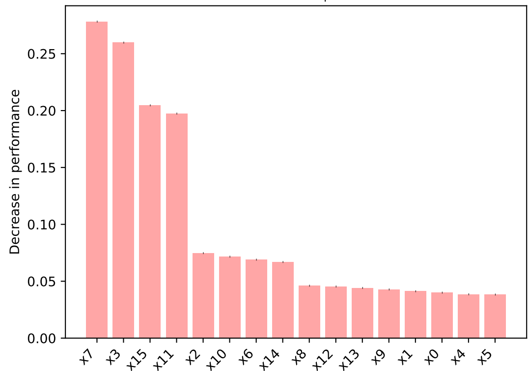
Permutation importance for RFR ep (NLO QCD, LHE, fiducial)
