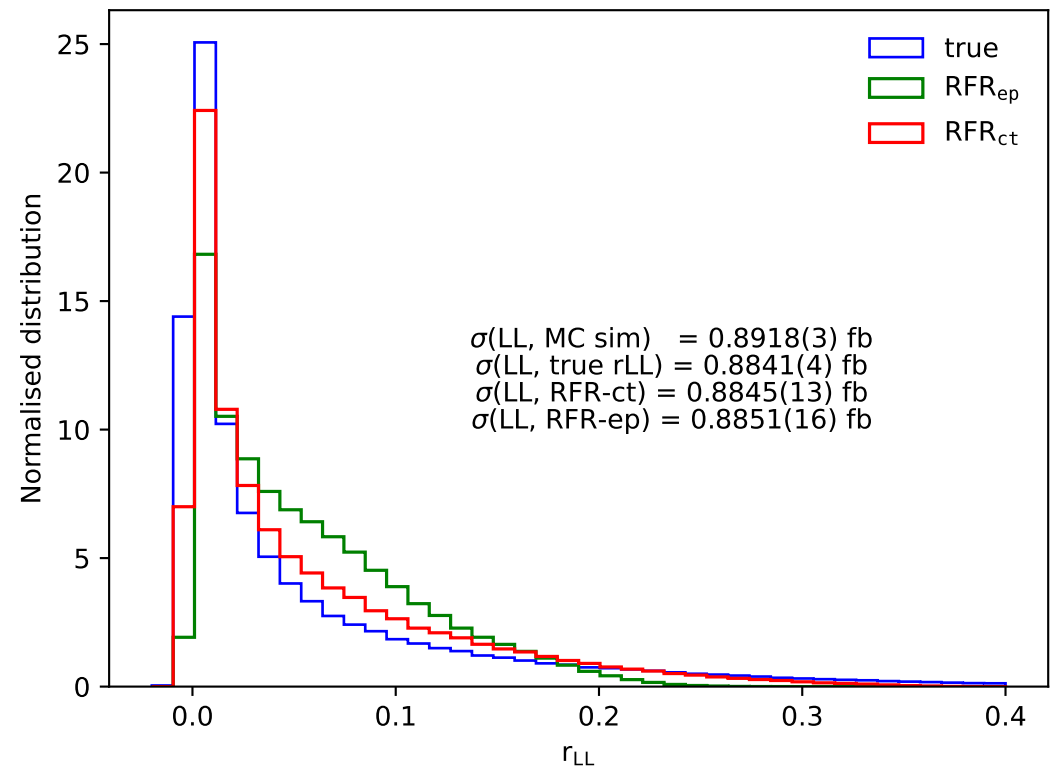
r_{LL} label (NLO QCD, LHE, fiducial)
