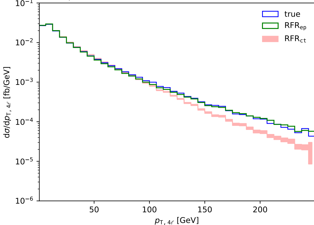
Four-lepton transverse momentum (NLO QCD, LHE, fiducial)
