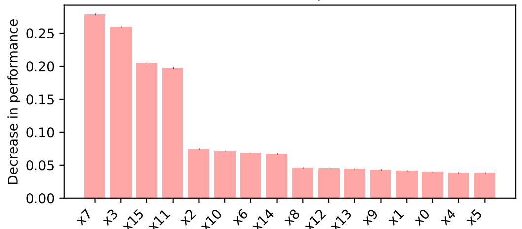
Permutation importance for RFR ep (NLO QCD, LHE, fiducial)
