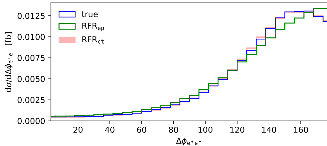
Positron-electron azimuthal separation (NLO QCD, LHE, fiducial)
