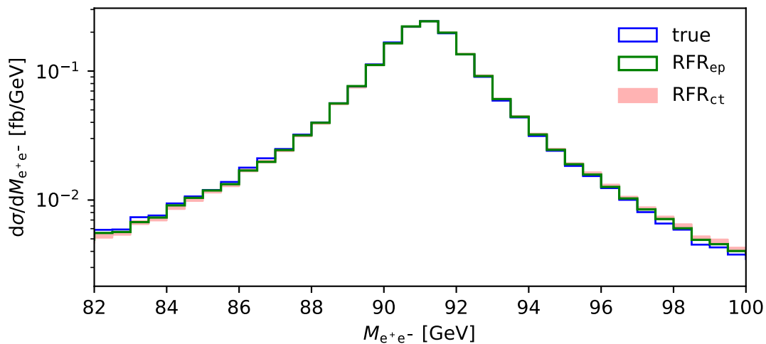
Positron-electron invariant mass (NLO QCD, LHE, fiducial)
