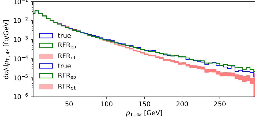
Four-lepton transverse momentum (NLO QCD, LHE, fiducial)
