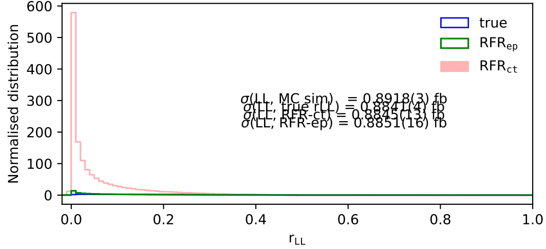
r_{LL} label (NLO QCD, LHE, fiducial)
