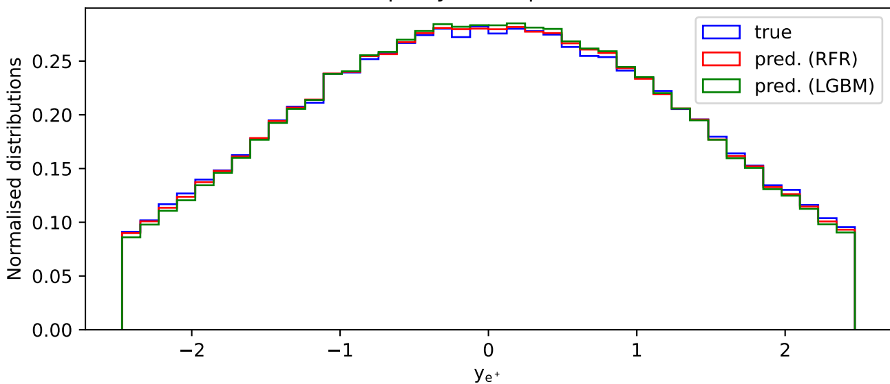
Rapidity of the positron
