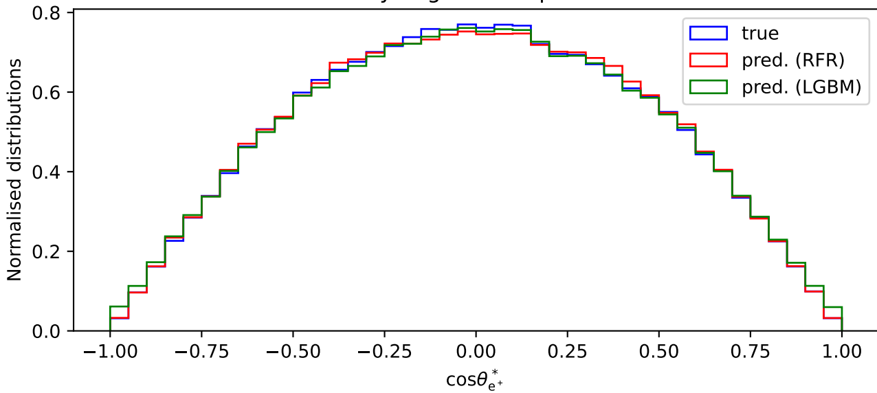
Decay angle of the positron
