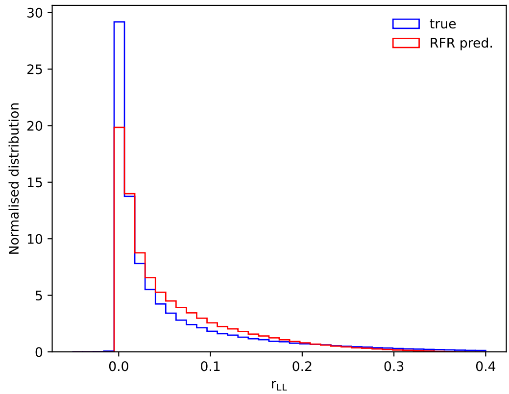
r_{LL} label (NLO QCD, LHE, fiducial)
