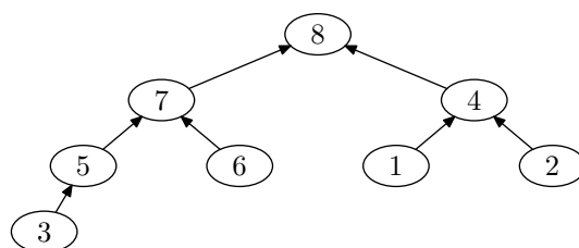
(j) After max-heapify on root again.
