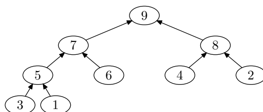
(h) After max-heapify on root again.
