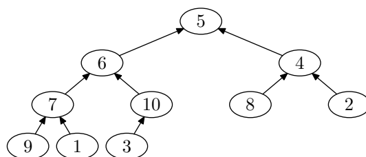
(b) After max-heapify on 5th node.
