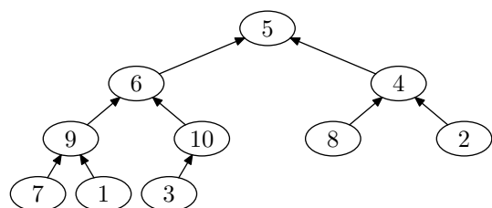
(c) After max-heapify on 4th node.
