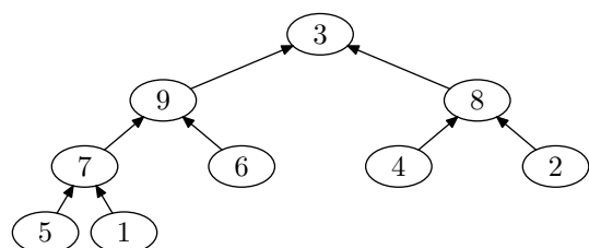
(g) Right after removing largest element 10.
