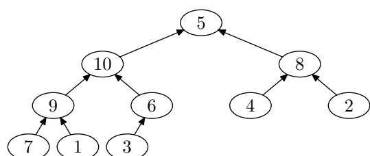
(e) After max-heapify on 2nd node.
