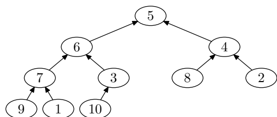
(a) Input array.
