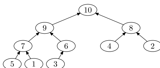
(f) After max-heapify on root node.
