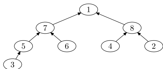
(i) Right after removing next-to-largest element 9.
