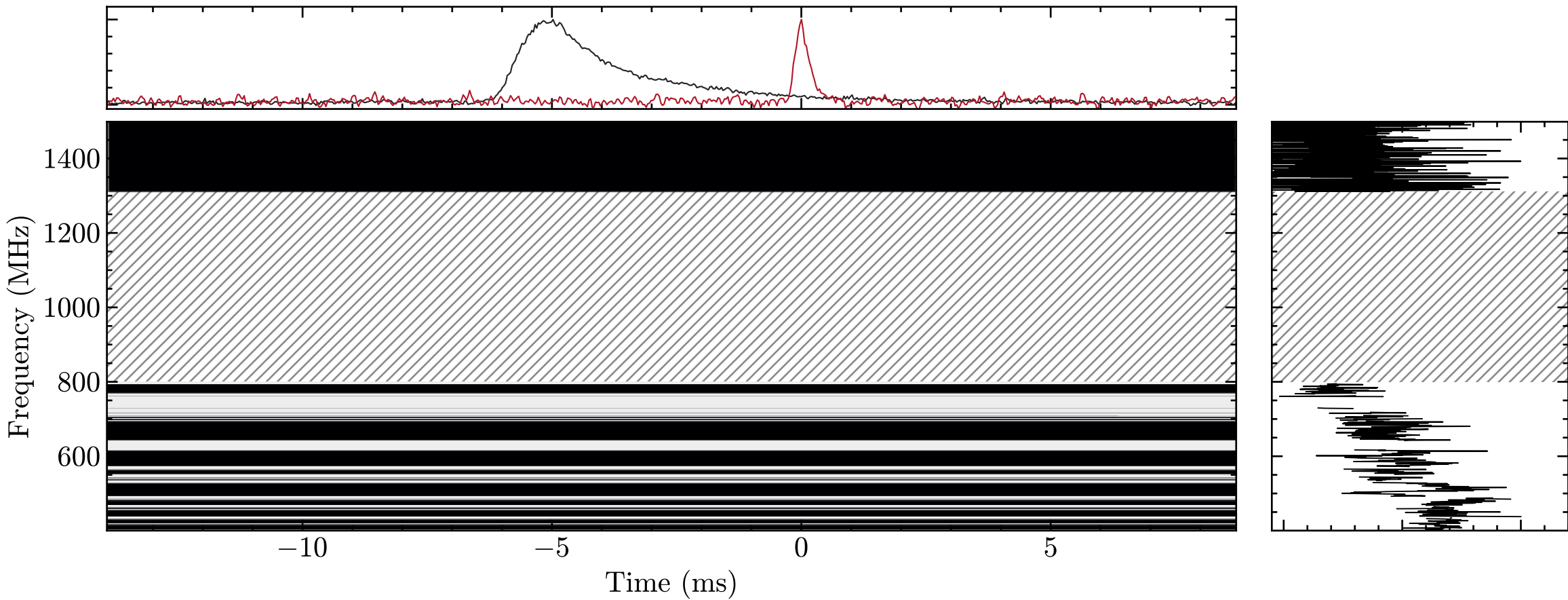
FRB 20240203A (no accepted joint fit)
