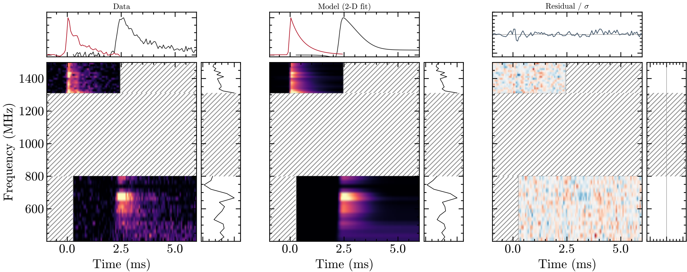
FRB 20230814B
