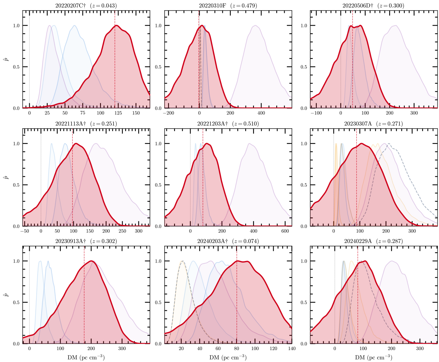
— P(\text{DM}_{\text{host}}) — MW halo — intervening system(s) — MW ISM (disk) — cosmic / IGM - - - intervening sightline sum
