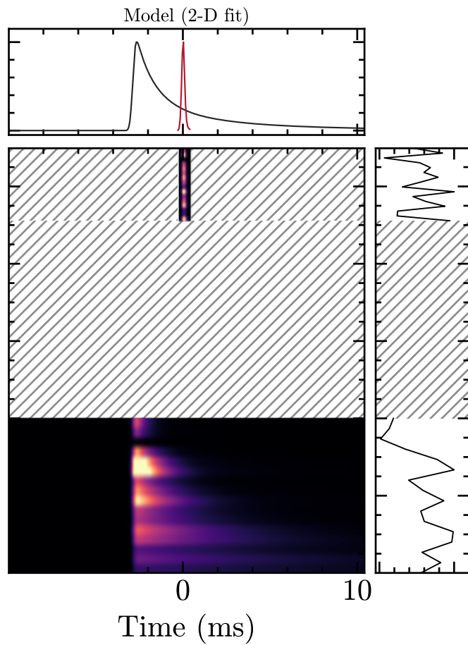
FRB 20240122A
