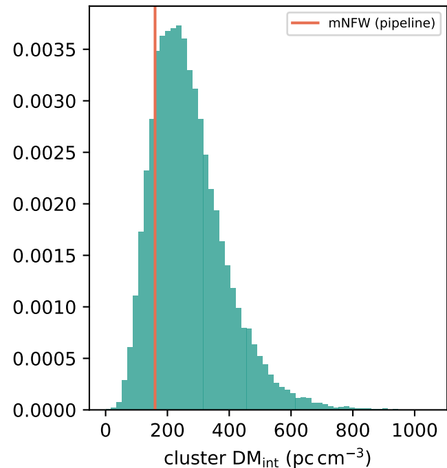
FRB 20230307A cluster column (beta-model MC)
