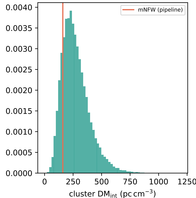
FRB 20230307A cluster column (beta-model MC)
