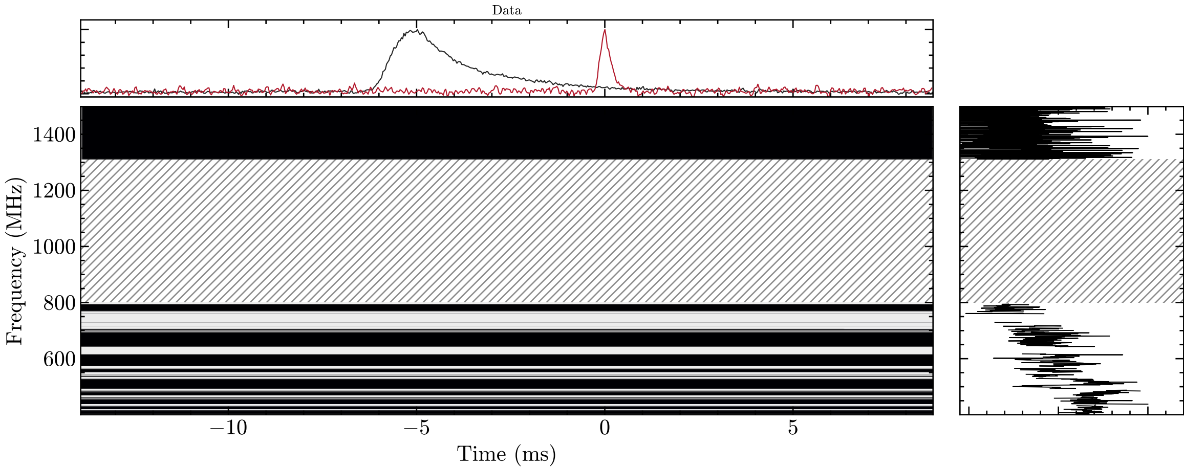
FRB 20240203A (no accepted joint fit)
