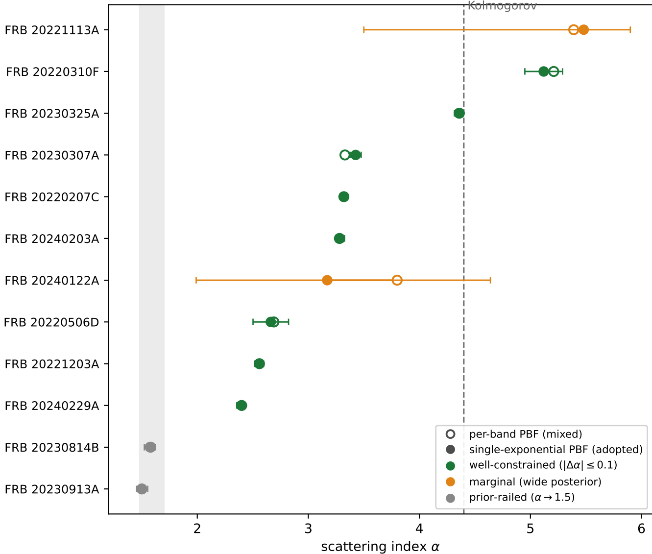
PBF systematic on the scattering index: per-band (open) \rightarrow single-exponential (filled)
