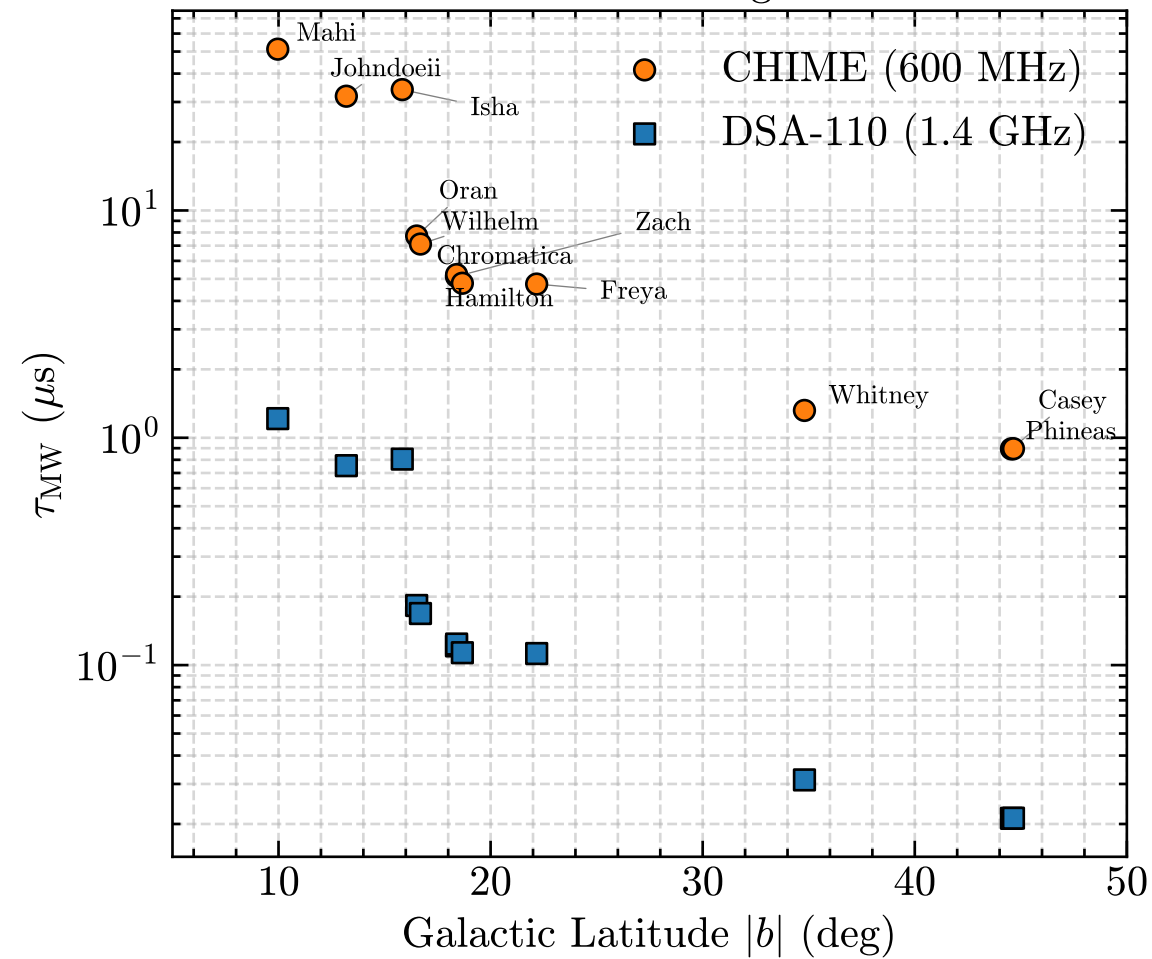
Galactic Scattering Floor
