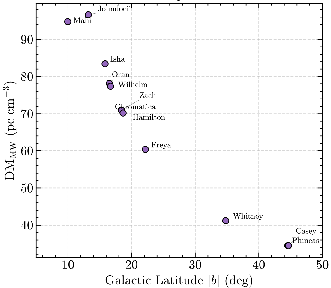
Galactic Dispersion Floor
