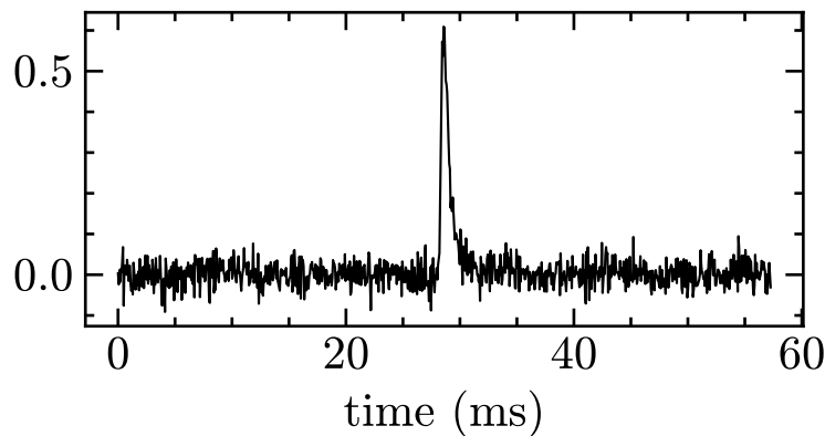
wilhelm 0.720-0.800 GHz w'rms=2.813 w'tail=22.369 ms
