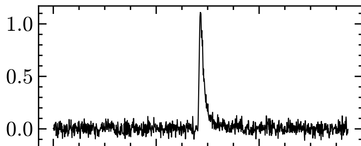
wilhelm 0.614-0.694 GHz w'rms=0.590 w'tail=1.142 ms
