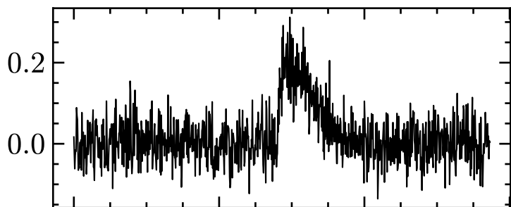
johndoeII 0.400-0.480 GHz w'rms=1.398 w'tail=25.304 ms
