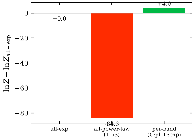
joint-fit evidence (wilhelm C1D1)
