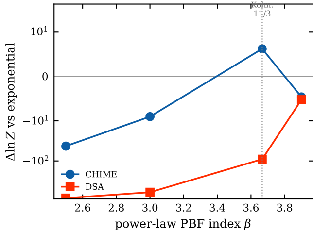
per-band PBF preference
