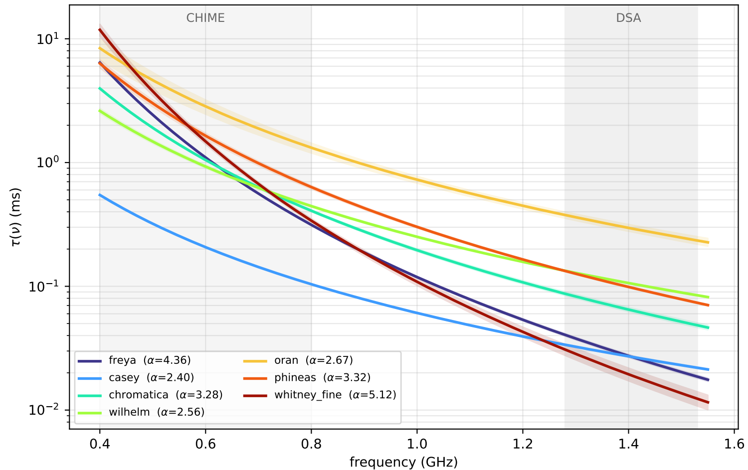
All-exp joint-fit \tau(\nu) = \tau_{1\text{GHz}} \nu^{-\alpha} ladder (68% band)
