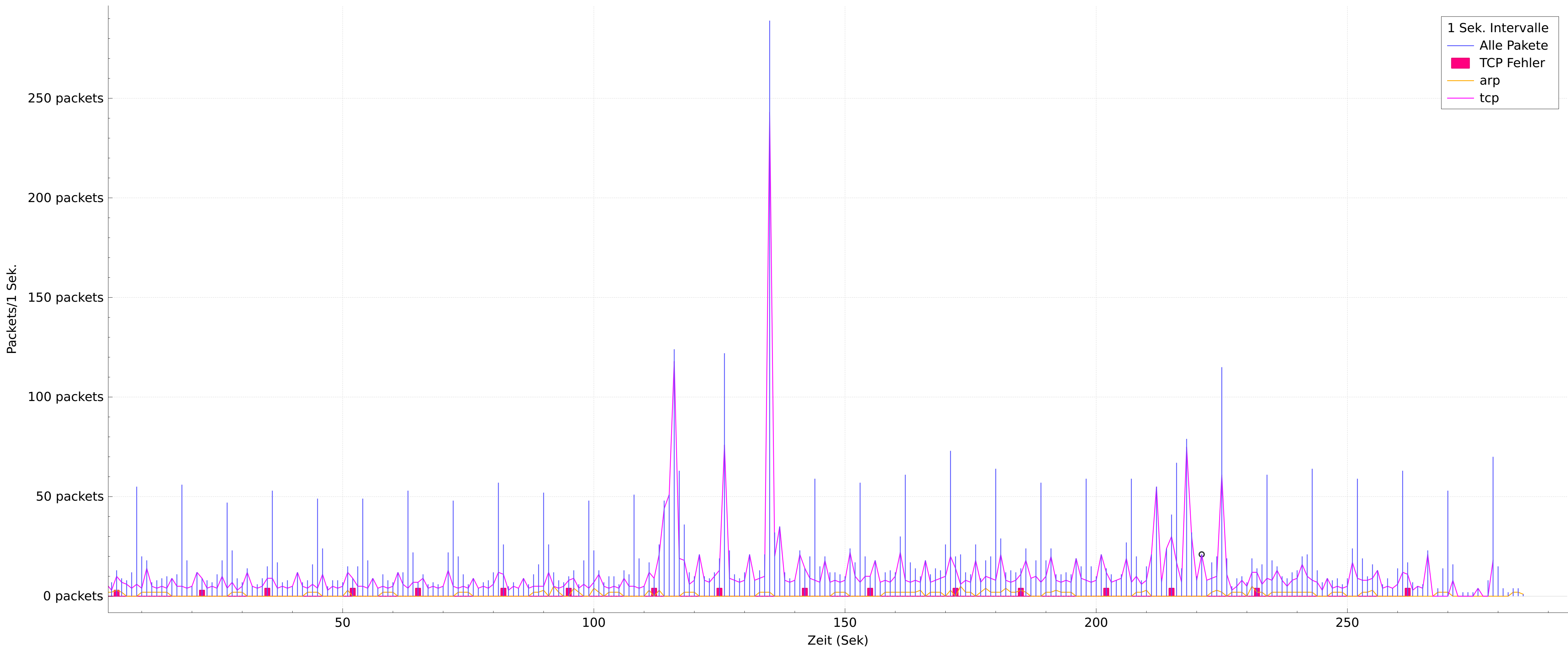
Wireshark I/O Graphen: attack6.pcapng
