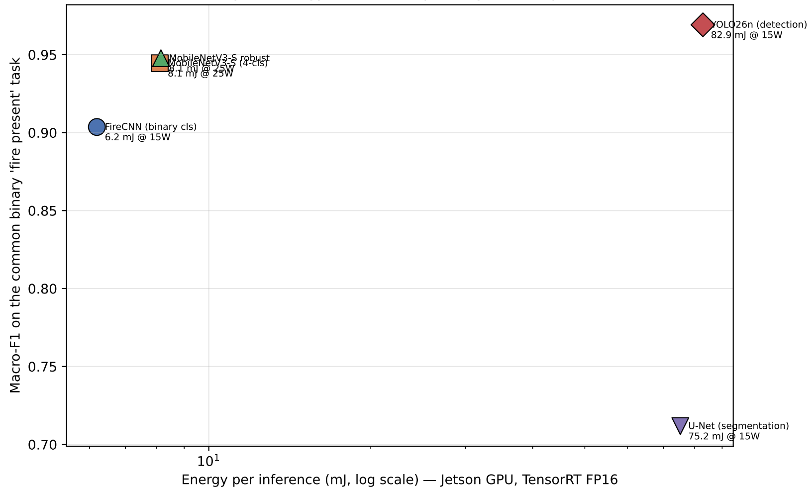
Accuracy vs energy: what each paradigm costs per frame
