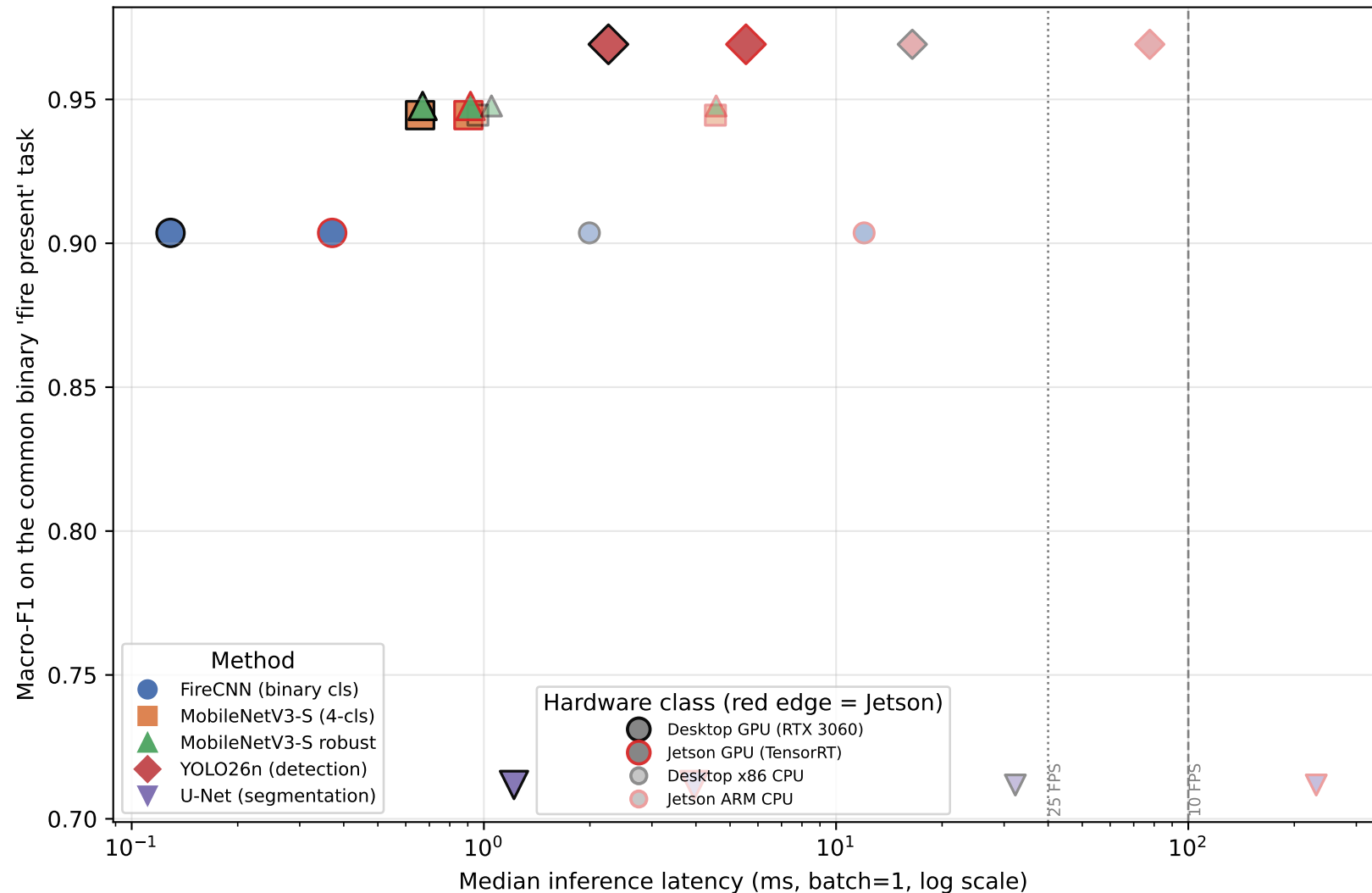
Accuracy vs inference cost across detection paradigms
