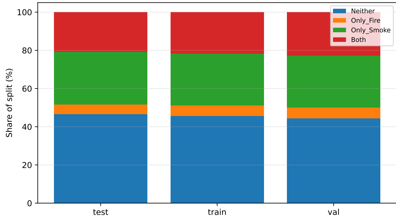
Class distribution is stable across splits (Only_Fire is 5.4% overall)
