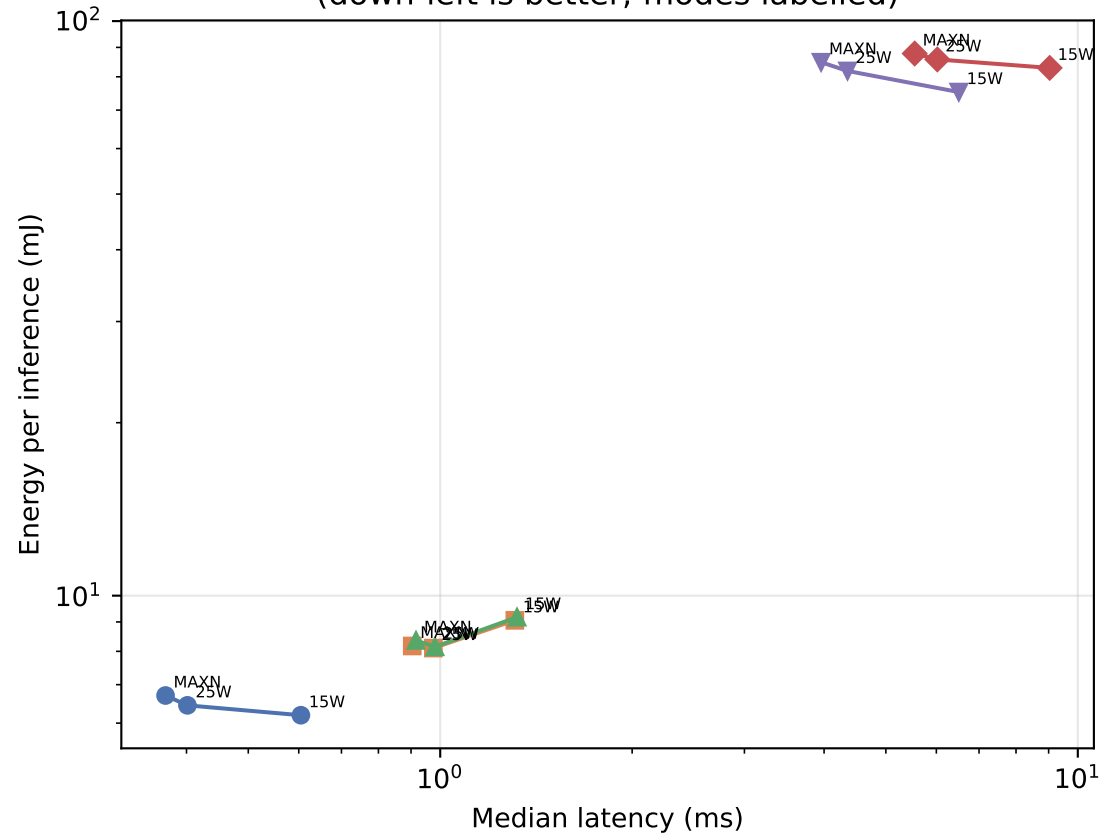
Latency vs energy trade-off (down-left is better; modes labelled)
