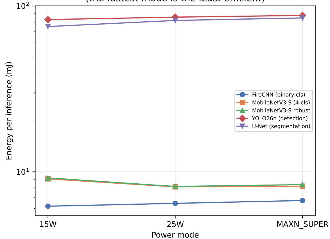
Energy rises with power mode (the fastest mode is the least efficient)
