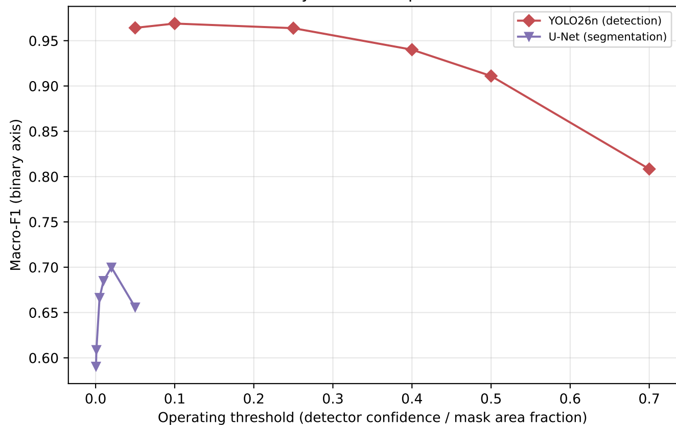
Sensitivity to the collapse threshold
