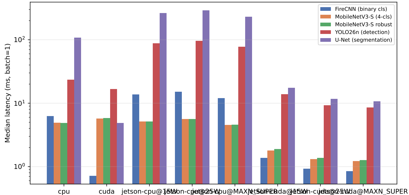
Inference latency by device (FP32, lower is better)
