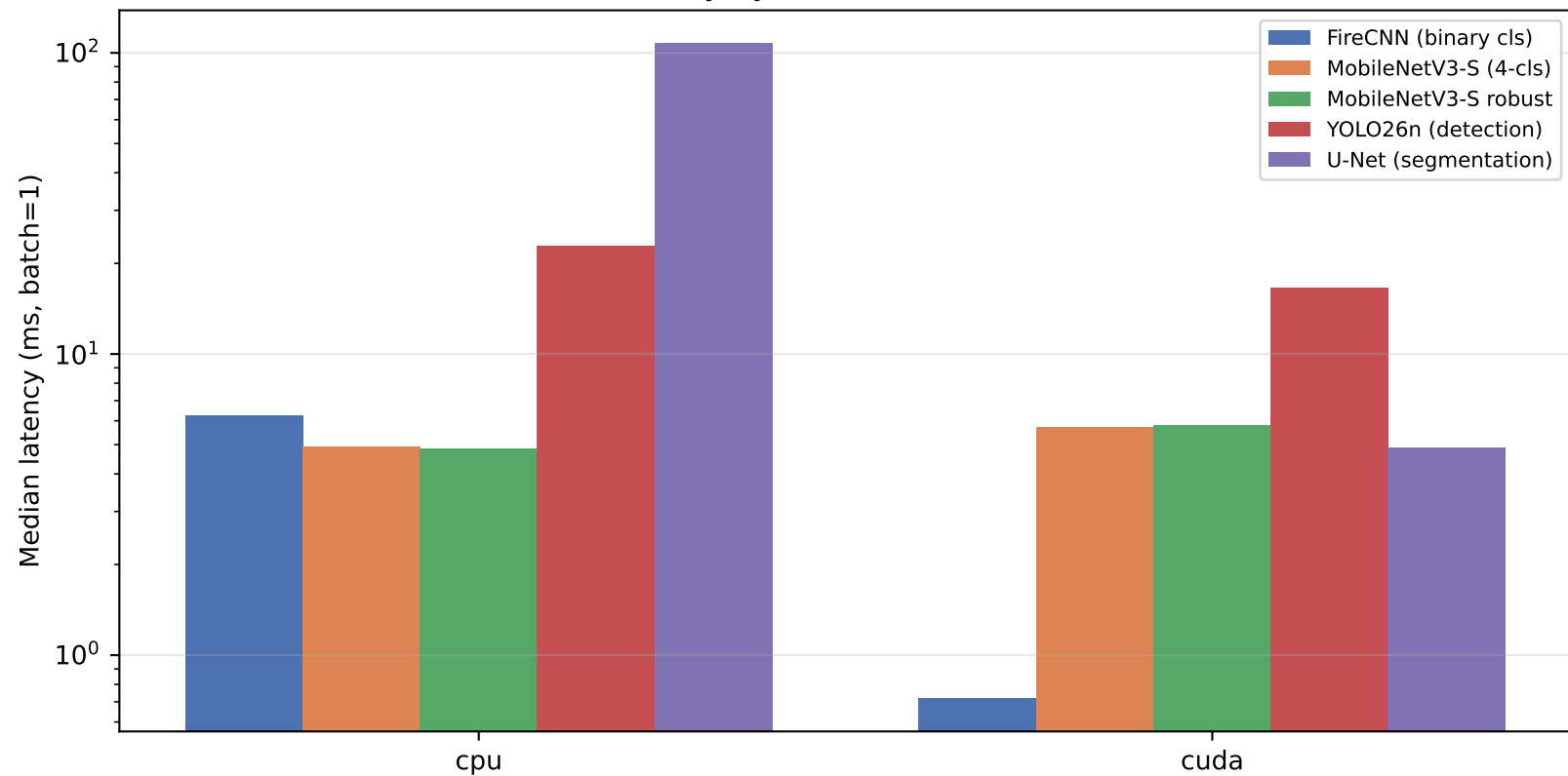
Inference latency by device (FP32, lower is better)
