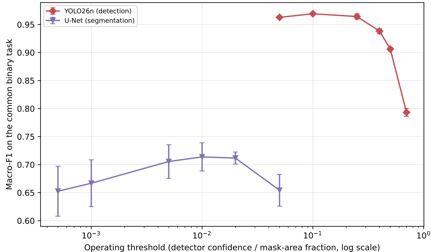
Sensitivity to the collapse threshold seeded checkpoints, mean \pm std (up to 5 seeds per point)
