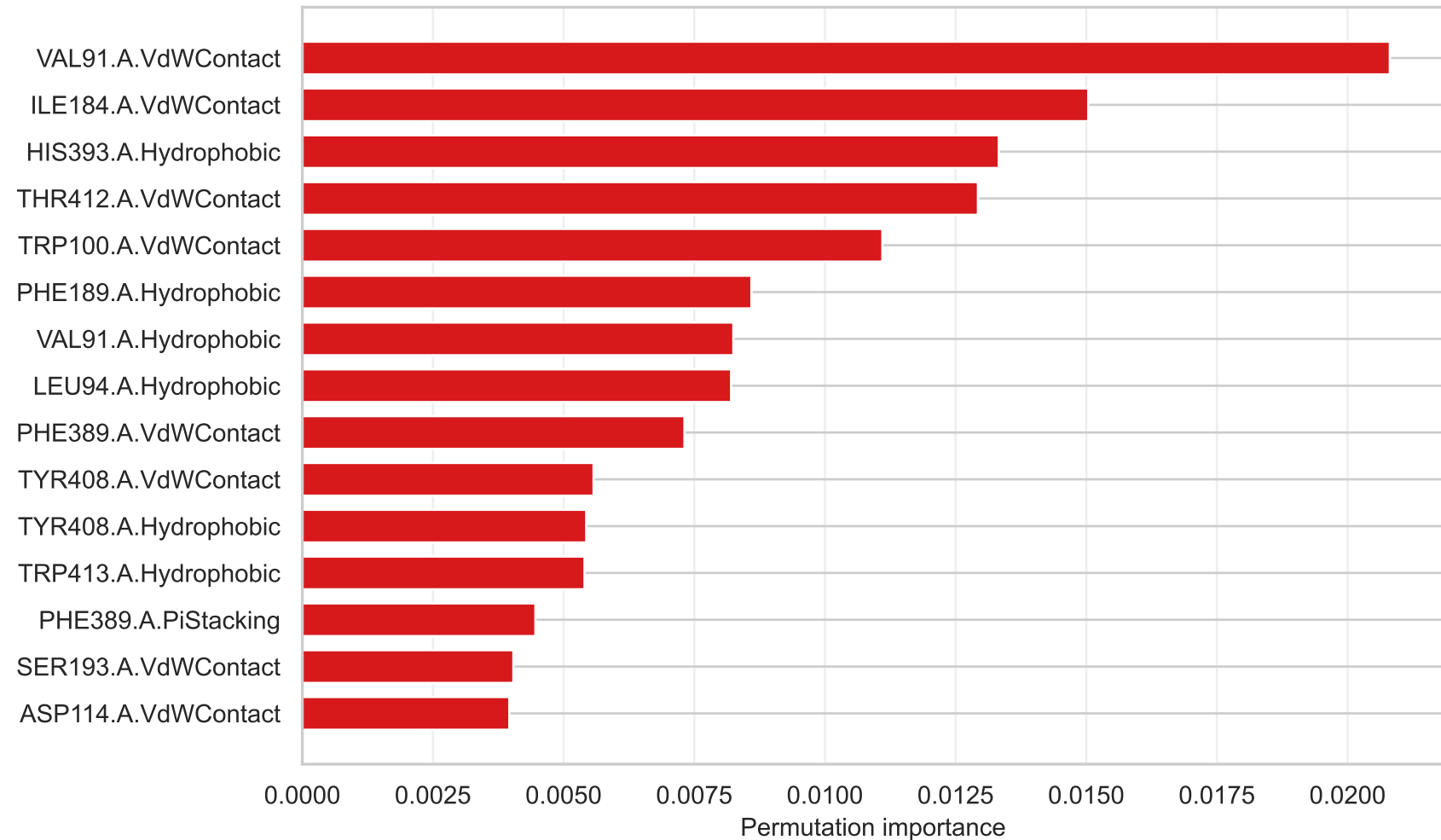
D2 – Top-15 cech (Permutation importance)
