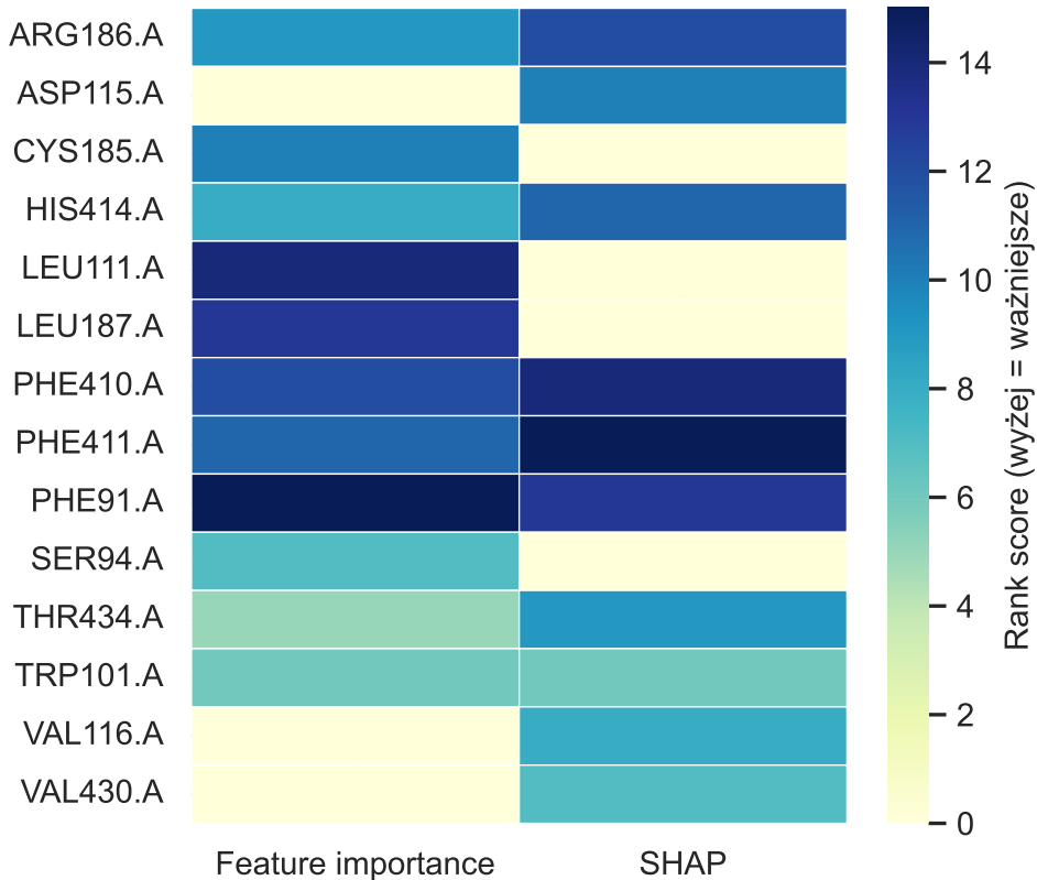
D4 – Feature importance vs SHAP (top-15)
