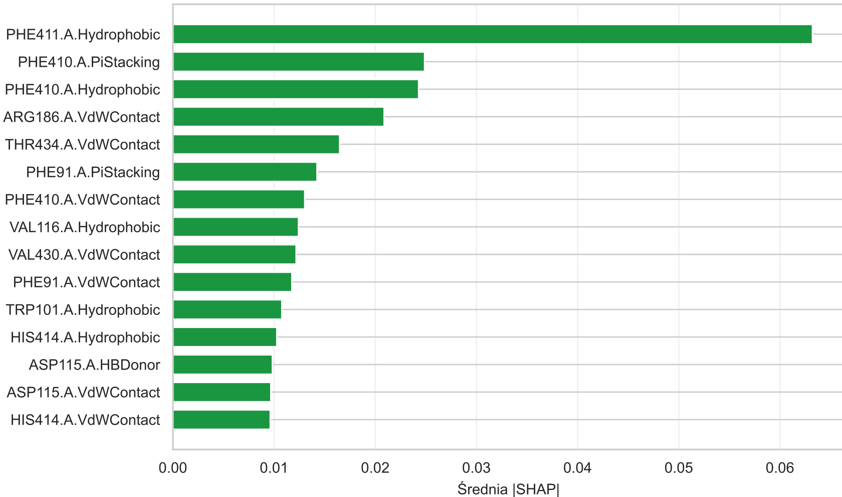
D4 – Top-15 cech (SHAP)
