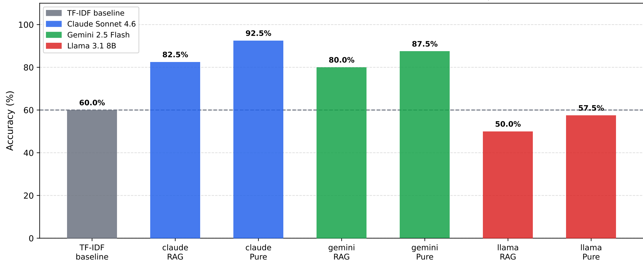
TF-IDF Cosine Baseline vs. LLM-as-a-Judge (same 40-case test set, same bucket thresholds: \geq 0.65 correct, \geq 0.30 partial)
