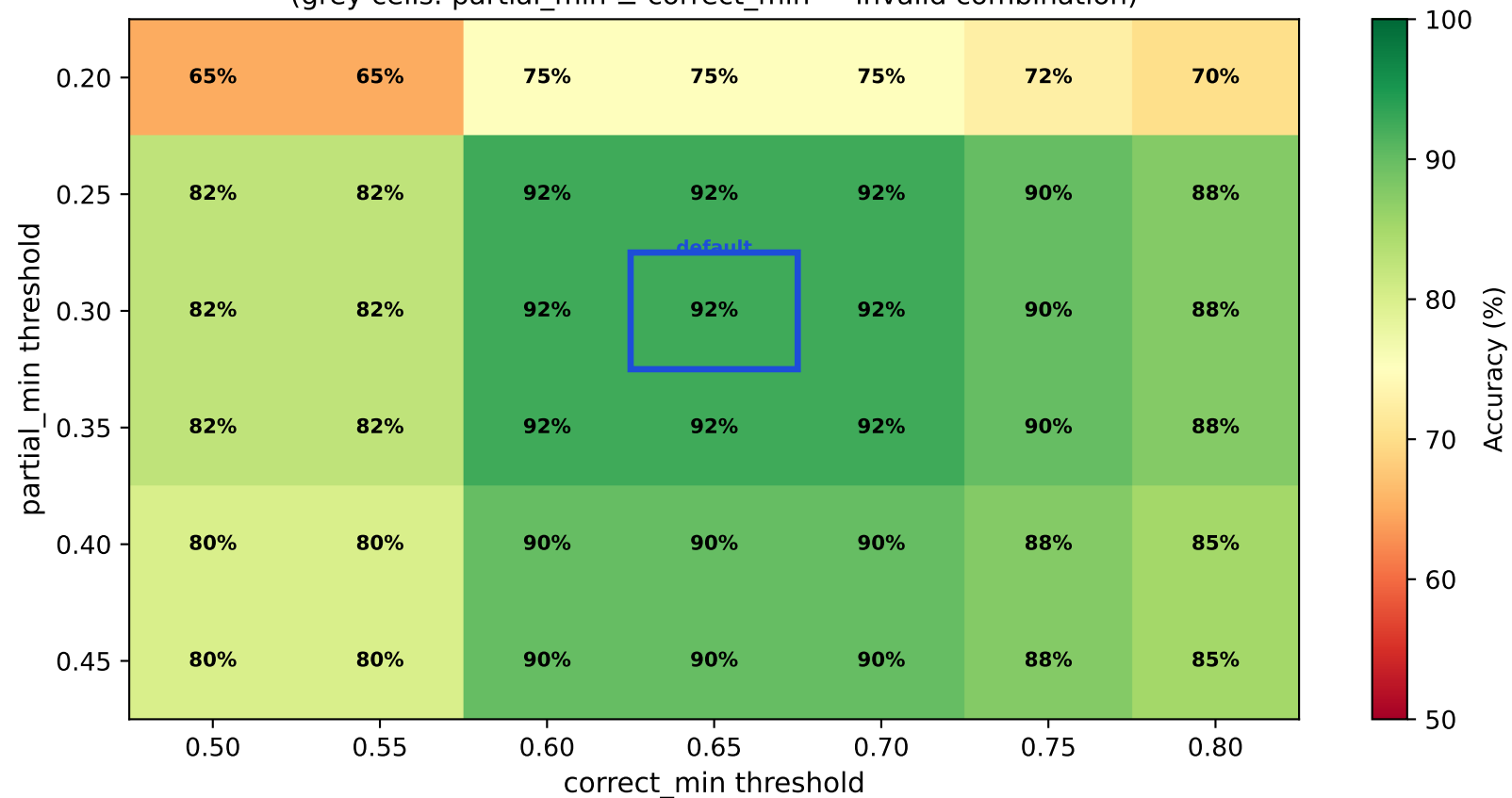
Threshold Sensitivity — claude · Pure (grey cells: partial_min \geq correct_min — invalid combination)
