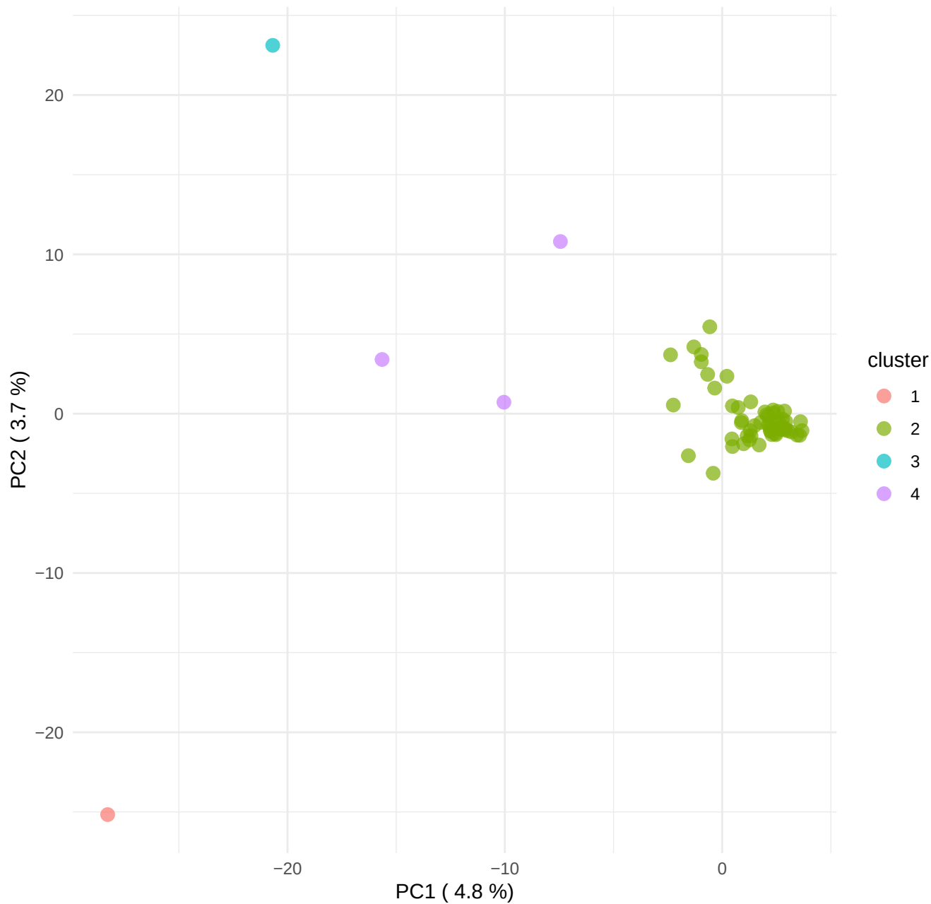
K-means (BoW), k = 4 - PCA
