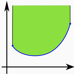
Convex function
