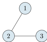
Node-link diagram
