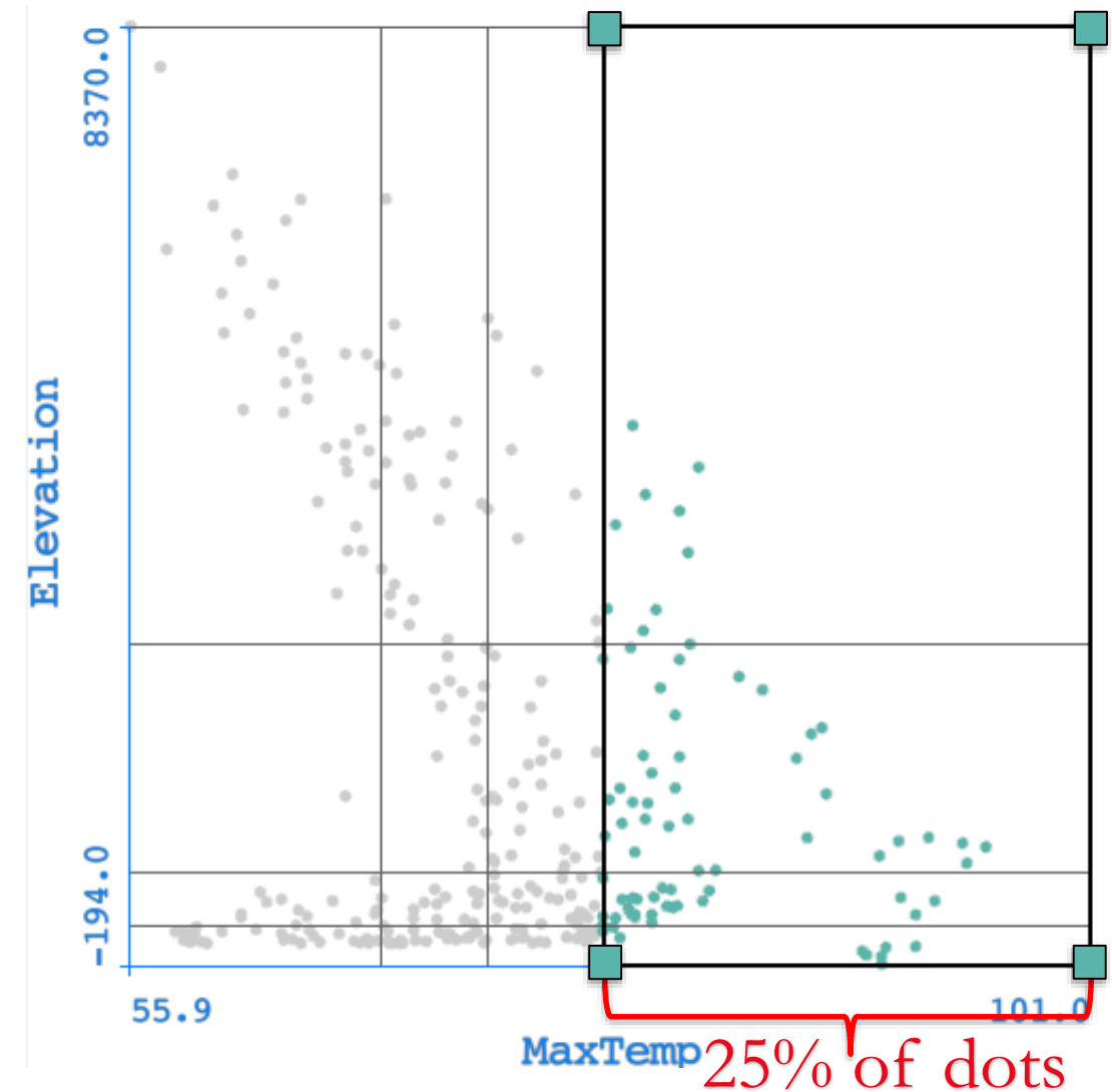
Percentile grid (rank-based)
