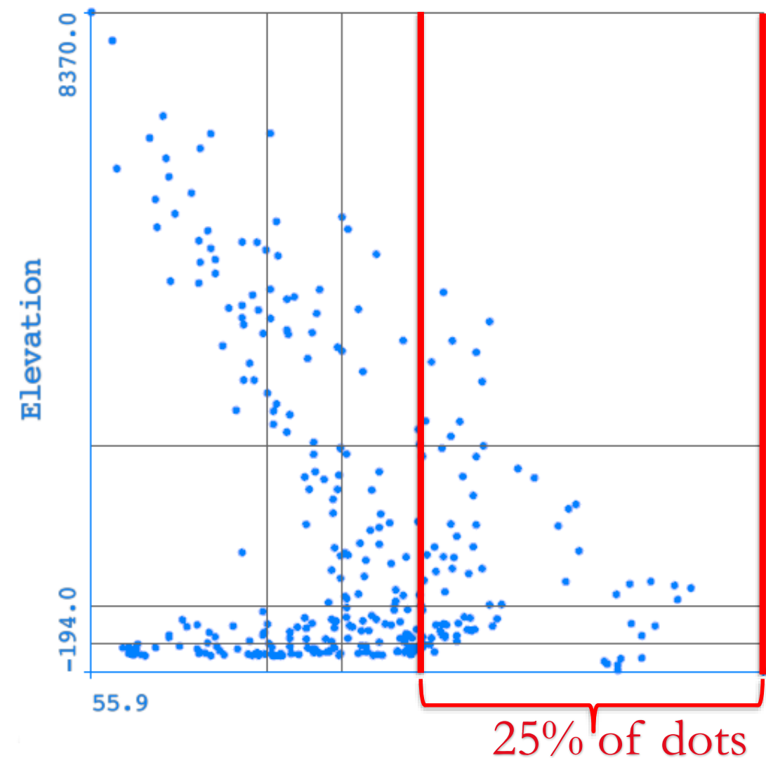
Percentile grid (rank-based)
