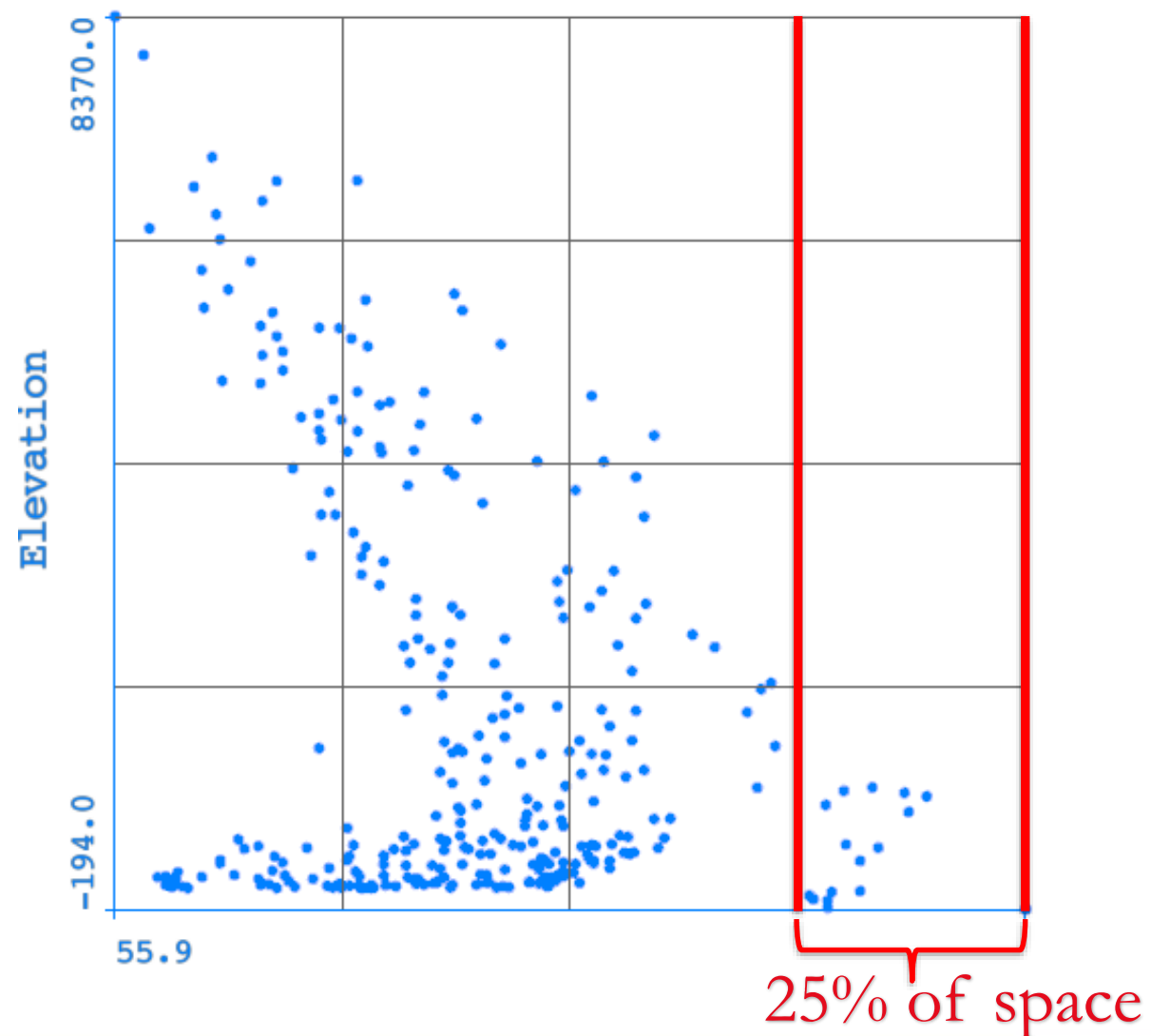
Regular grid (value-based)
