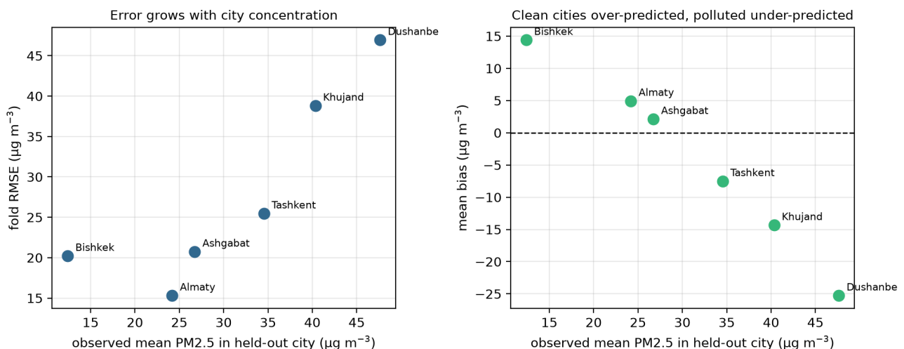
Figure 3. Leave-city-out error against the held-out city's mean PM2.5. Left: fold RMSE rises with city concentration (Spearman \rho = +0.94 ). Right: mean bias falls monotonically from +14.9 \mu\text{g}/\text{m}^3 in Bishkek, the cleanest city, to -25.1 \mu\text{g}/\text{m}^3 in Dushanbe, the most polluted.
