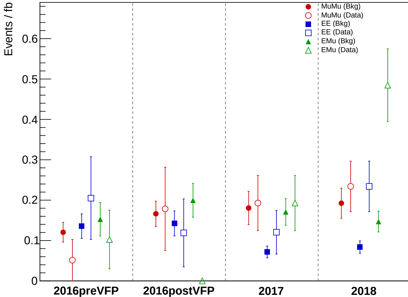
Total Background vs Data: PassCR1_BJet, HNL_ULIDv2
