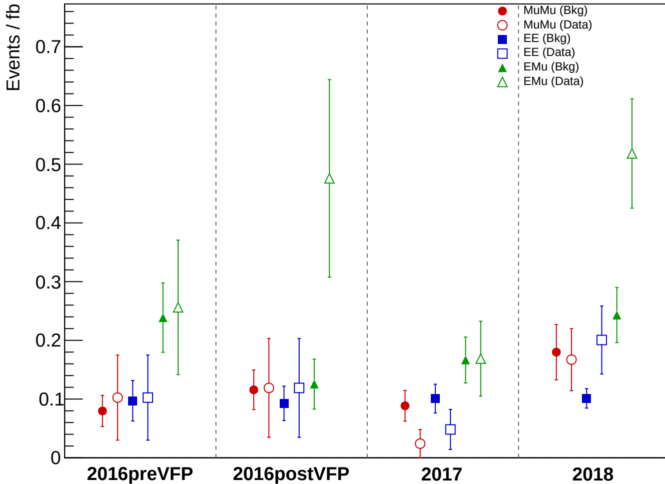
Total Background vs Data: PassCR2_BJet, HNL_ULIDv2
