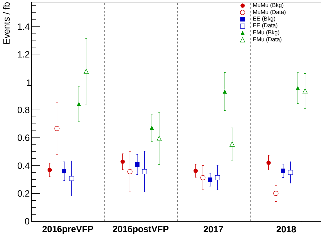
Total Background vs Data: PassCR2_MET, HNTightV2
