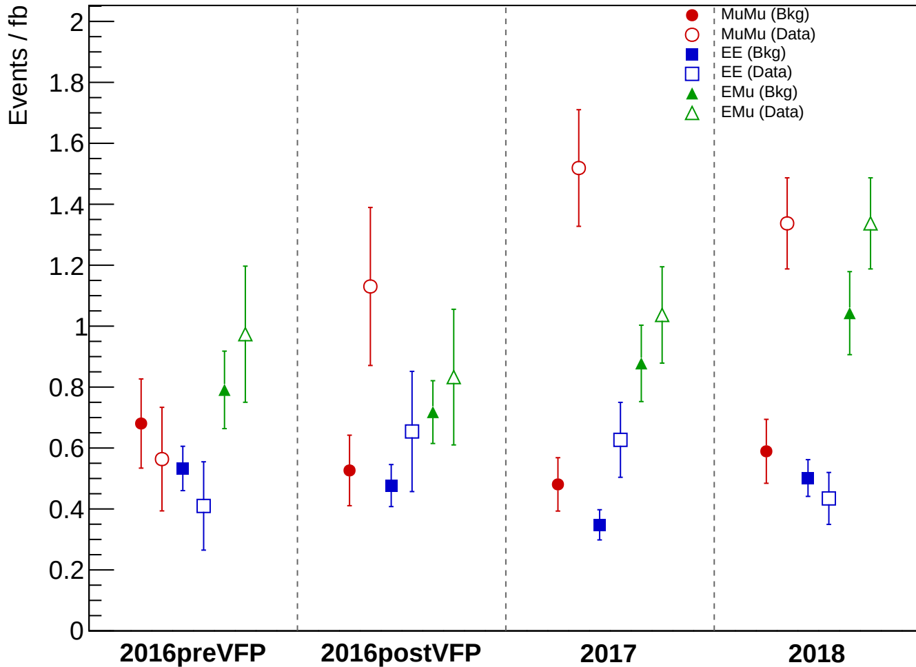
Total Background vs Data: PassCR2_MET, POGTight
