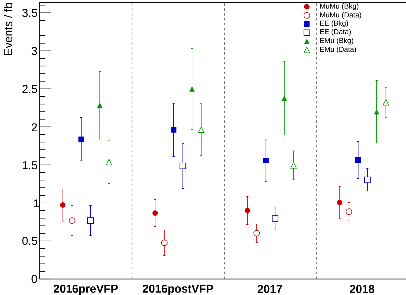
Total Background vs Data: PassCR3_BJet_HighJet, HNTightV2
