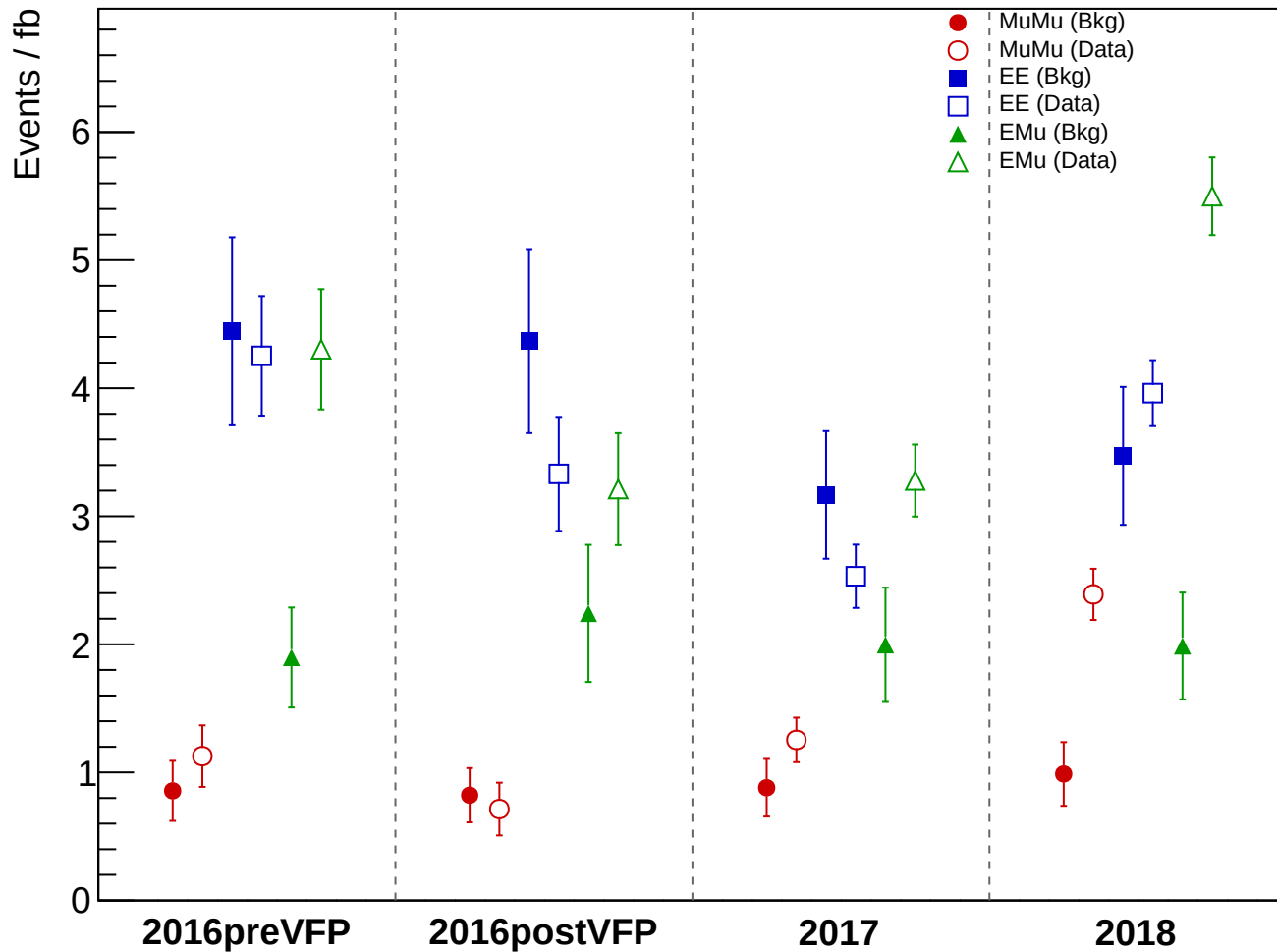
Total Background vs Data: PassCR3_BJet_HighJet, POGTight
