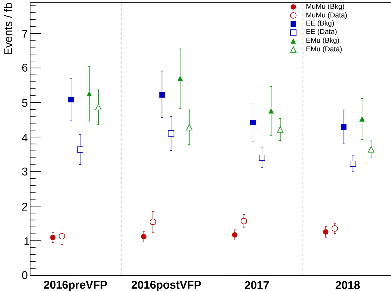
Total Background vs Data: PassCR3_MET_HighJet, POGTight
