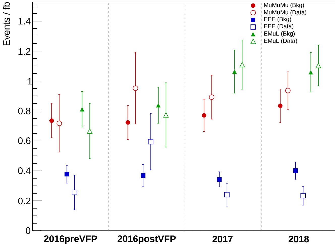
Total Background vs Data: HNL_WZVBF2_ThreeLepton_CR, POGTight
