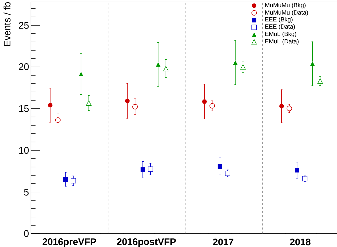
Total Background vs Data: HNL_WZ_SR3_ThreeLepton_CR, HNTightV2
