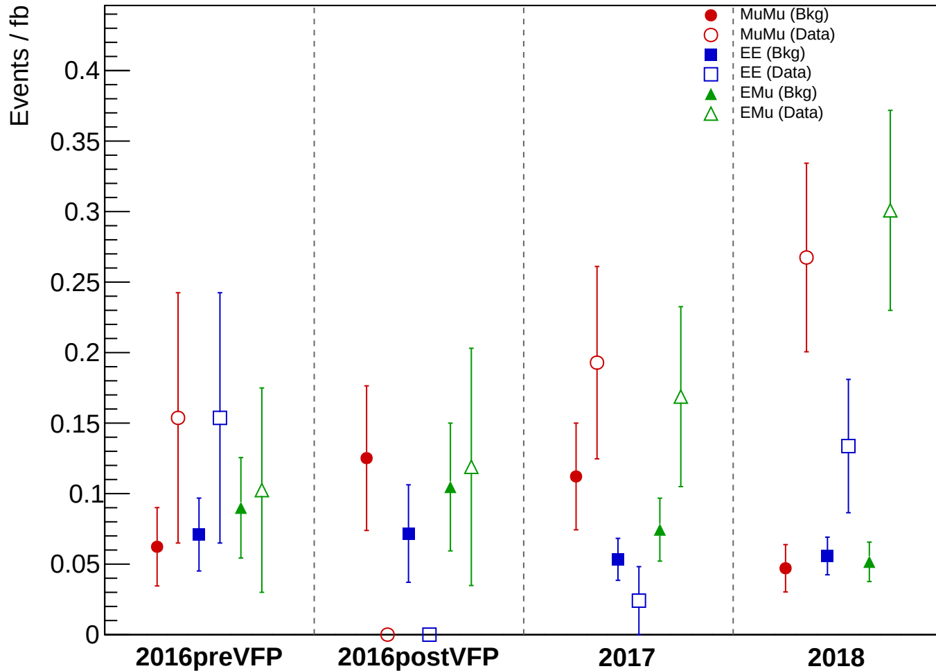
Total Background vs Data: PassCR1_BJet, POGTight
