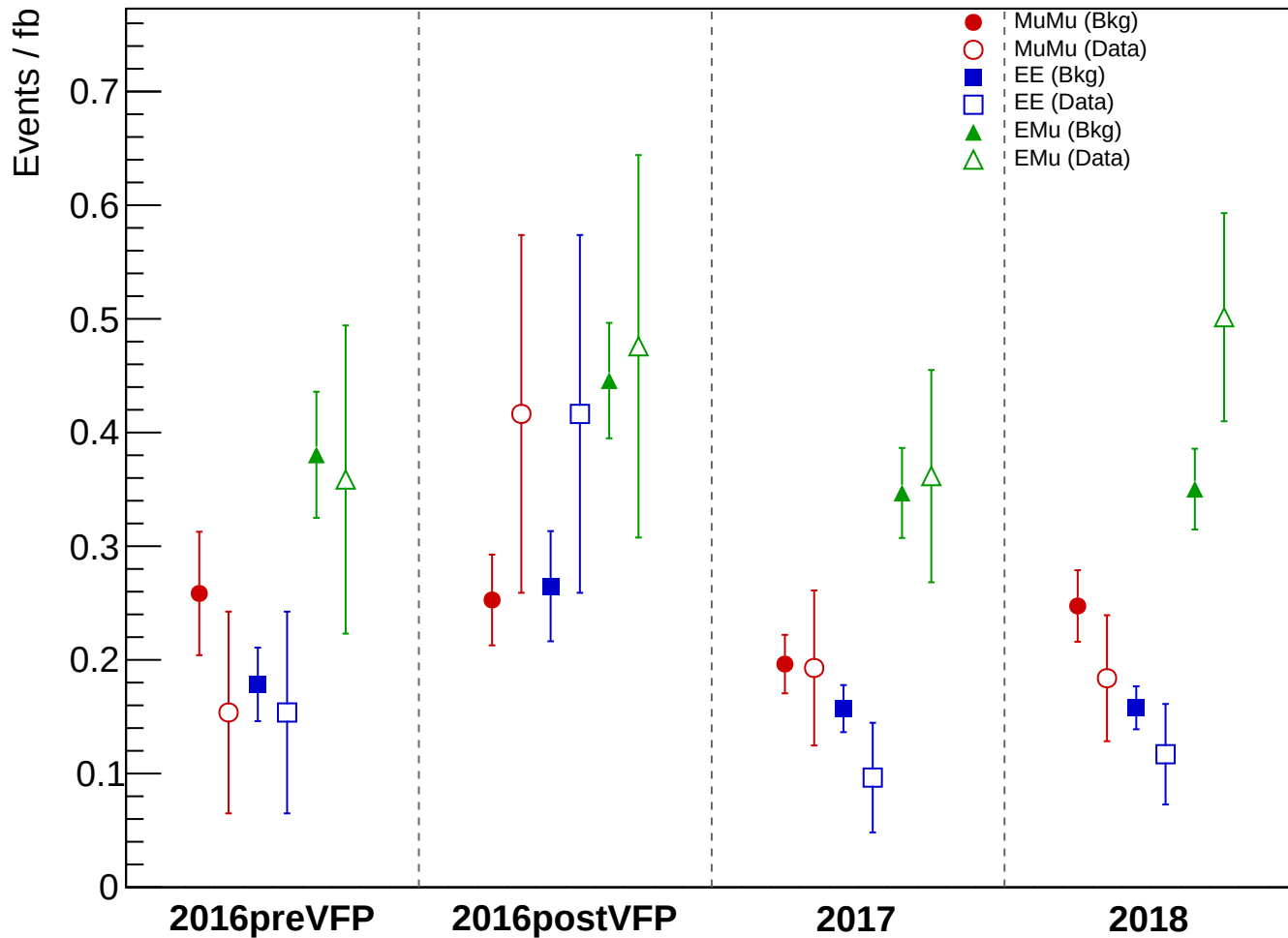
Total Background vs Data: PassCR1_MET, HNL_ULIDv2
