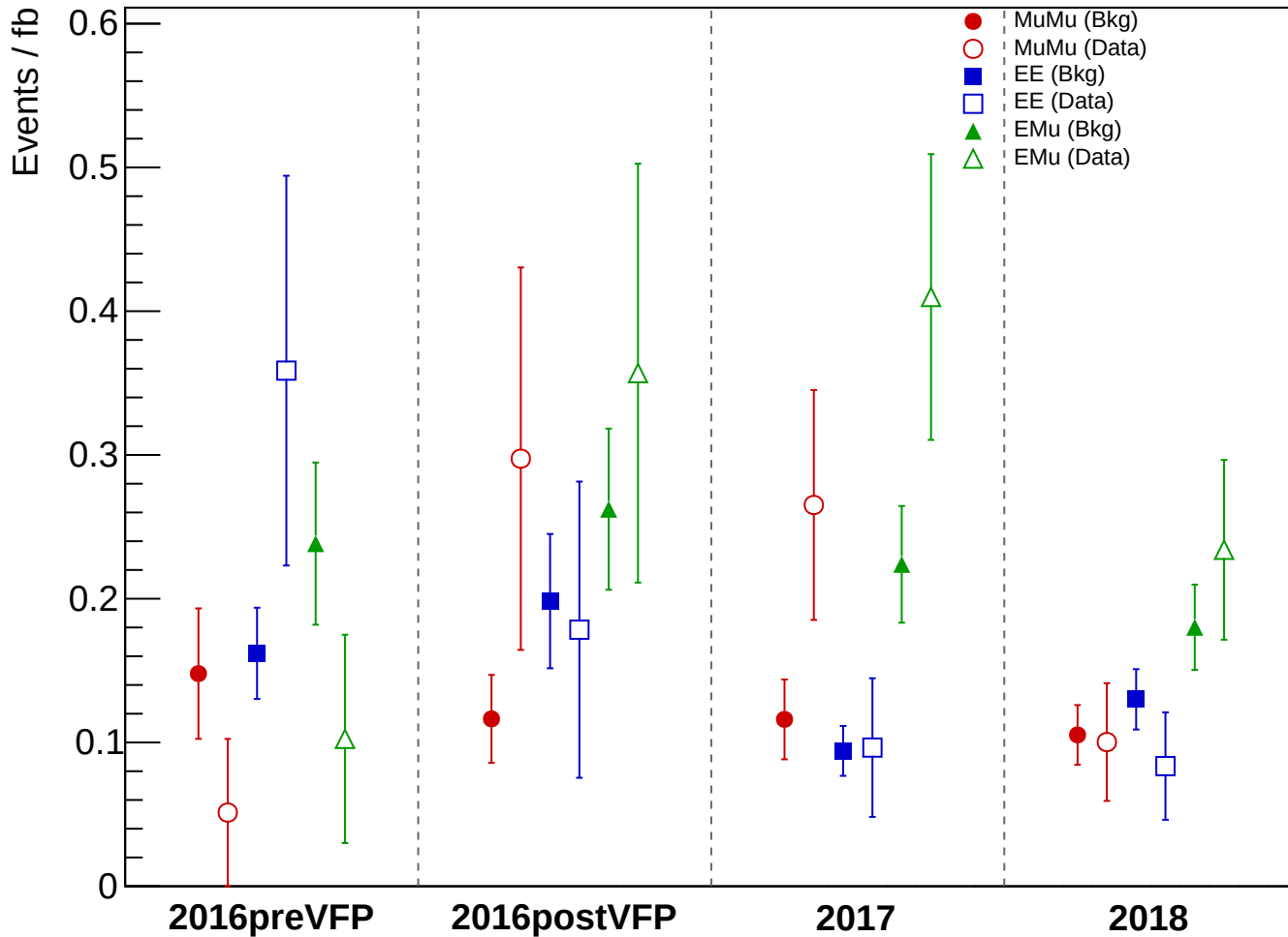
Total Background vs Data: PassCR1_MET, POGTight
